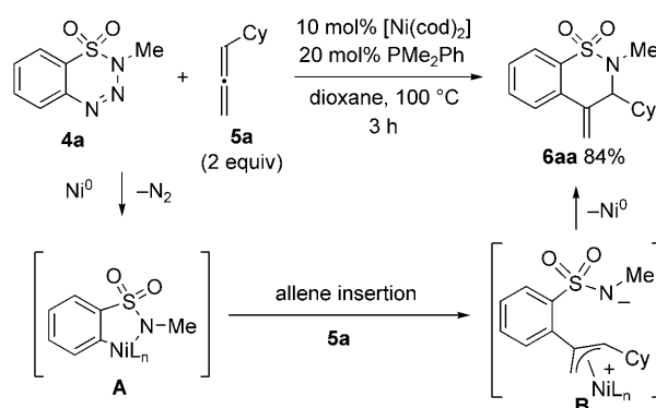
Scheme 2. Ni 0 -catalyzed denitrogenative annulation using achiral phosphine. cod = 1,5-cyclooctadiene.
