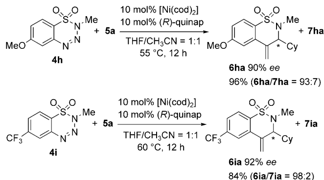
Scheme 3. Ni 0 -catalyzed enantioselective annulation: Scope of the substituent on the benzene ring of 4 .
