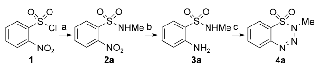
Scheme 1. a) NH 2 Me, Et 3 N, CH 2 Cl 2 , RT, 36 h, 89%; b) Zn, NH 4 Cl, MeOH, RT, 6 h, 96%; c) NaNO 2 , HCl, EtOH, 0°C, 9 h, 82%.
